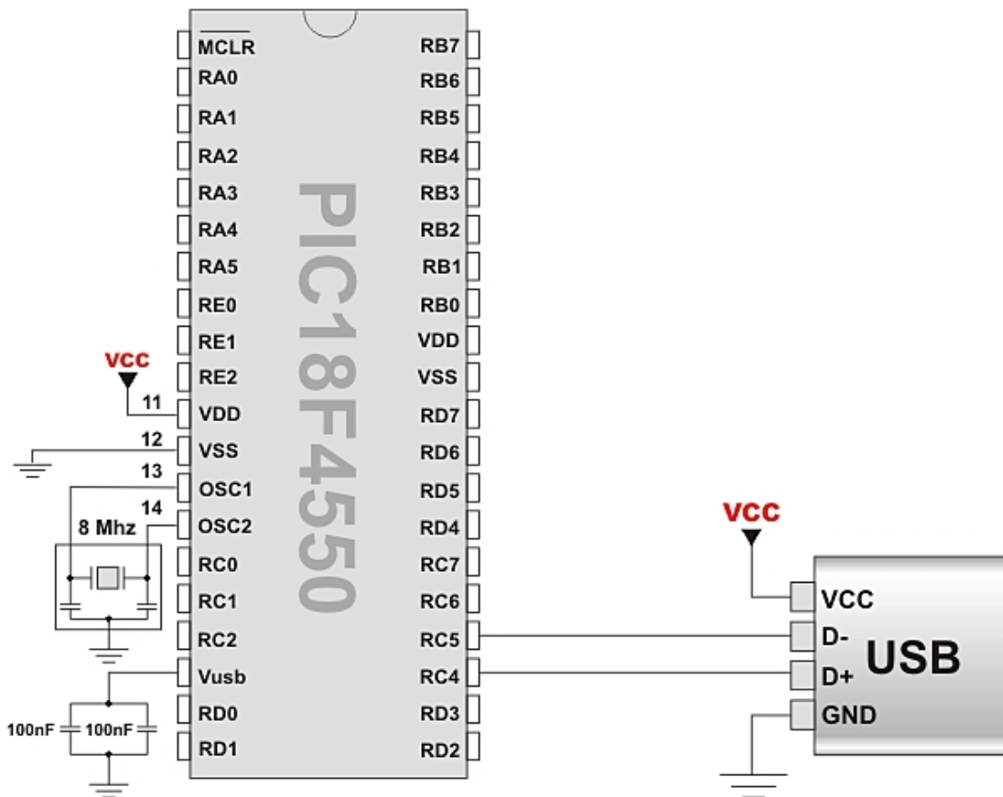
USB connection scheme
